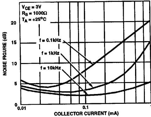
FIGURE 9. TYPICAL NOISE FIGURE vs COLLECTOR CURRENT
