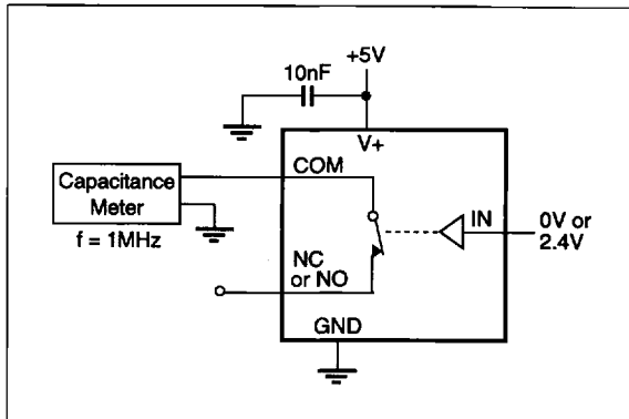
Figure 8. Channel-On Capacitance
