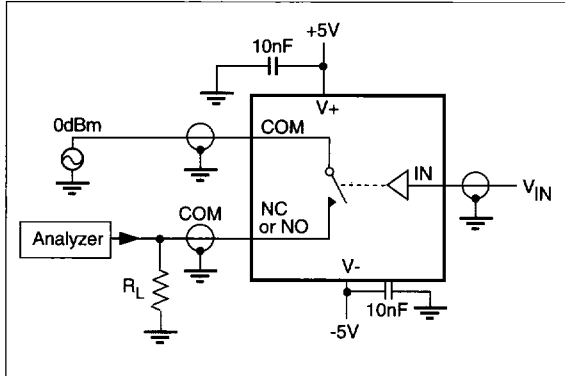
Figure 5. Off Isolation
