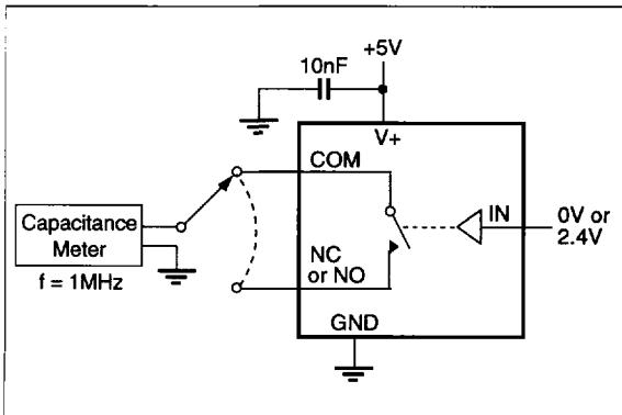
Figure 7. Channel-Off Capacitance
