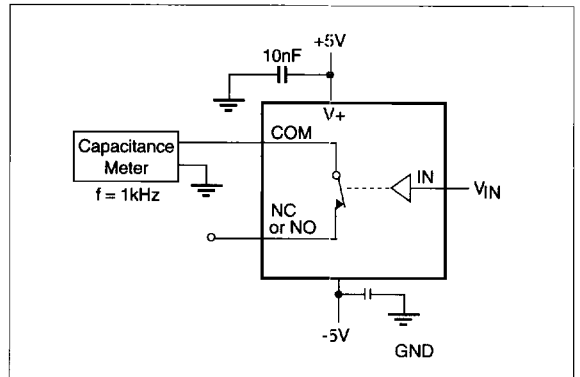
Figure 8. Channel-On Capacitance
