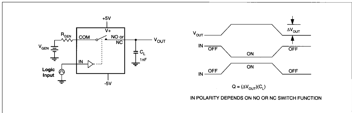
Figure 4. Charge Injection
