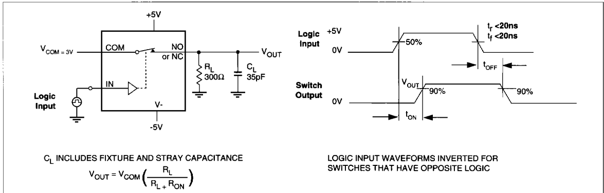
Figure 2. Switching Time
