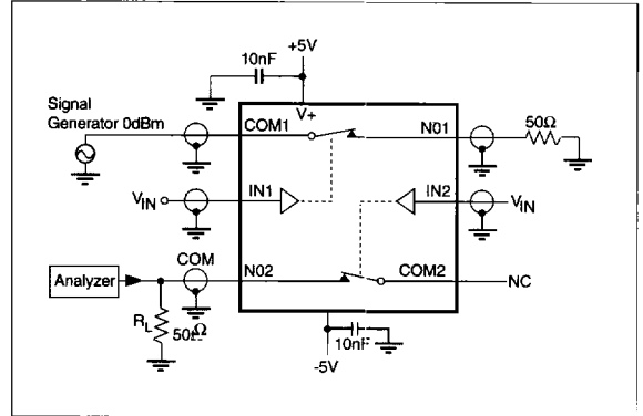
Figure 6. Crosstalk
