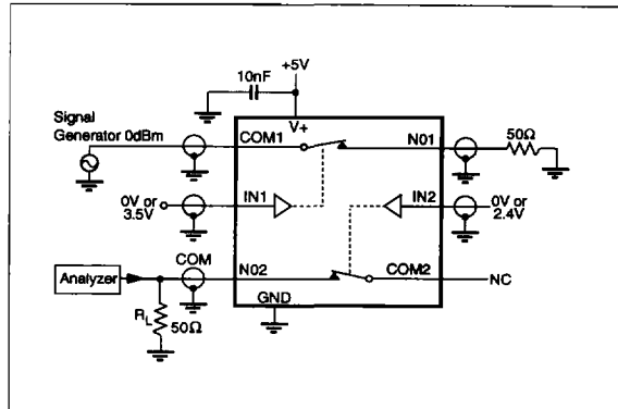
Figure 6. Crosstalk
