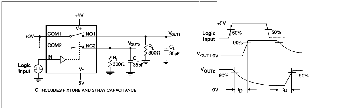
Figure 3. Break-Before-Make Interval (PS322 only)
