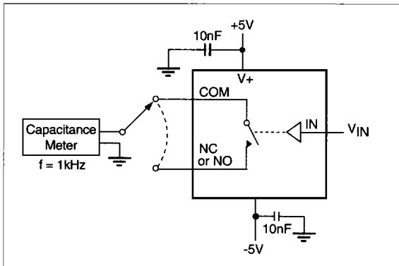
Figure 7. Channel-Off Capacitance
