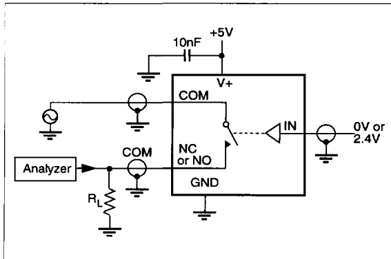
Figure 5. Off Isolation
