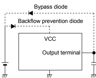
Fig.27 Bypass Diode
