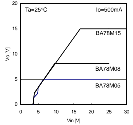
Fig.3 Line Regulation (Io=500mA)
