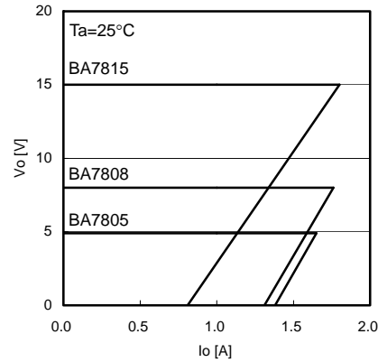
Fig.17 Load Regulation
