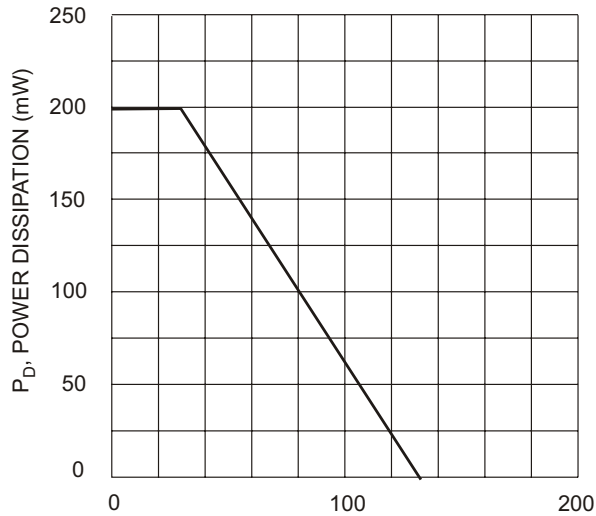
P_D , POWER DISSIPATION (mW) T_A , AMBIENT TEMPERATURE (°C) Fig. 5 Power Derating Curve, Total Package
