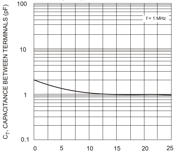
C_T , CAPACITANCE BETWEEN TERMINALS (pF) Fig. 3 Typical Capacitance Between Terminals Characteristics
