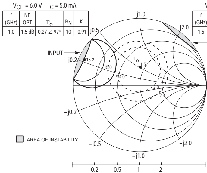
Figure 17. Constant Gain and Noise Figure Contours f = 1.0\text{ GHz}
