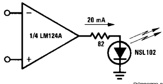
LED Driver
