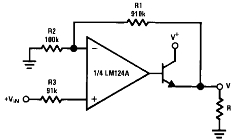
Power Amplifier
