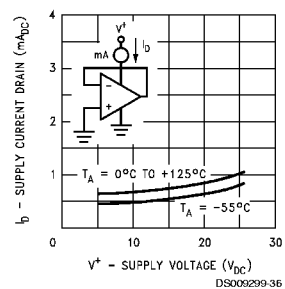
Supply Current
