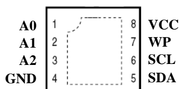
8-Lead UDFN
