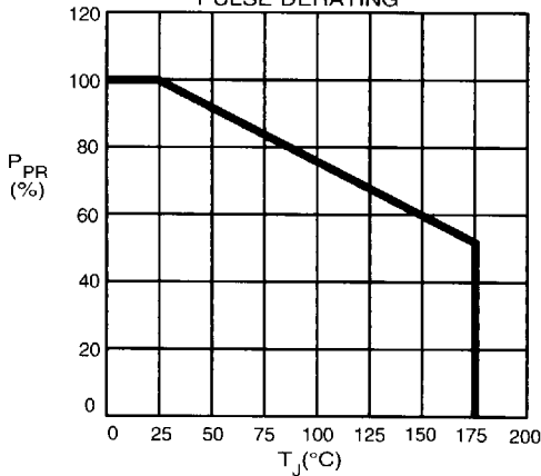
PULSE DERATING
