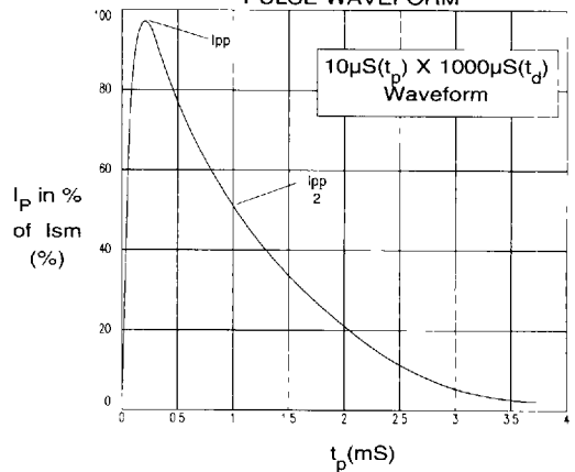
PULSE WAVEFORM
