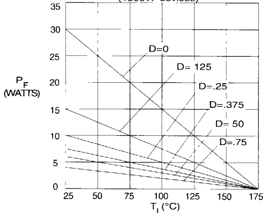
PULSE DERATING
