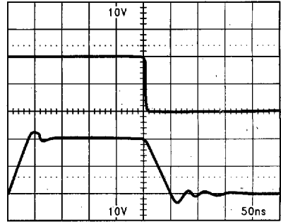
FIGURE 19. LH0032 Unity Gain Non-Inverting Large Signal Pulse Response: C_C = 5 pF, C_A = 1000 pF
