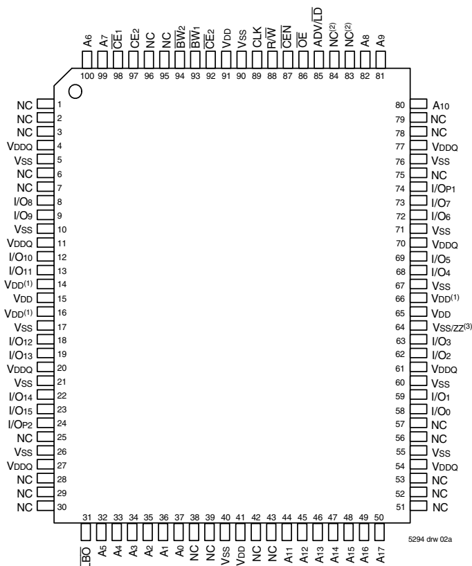
Top View 100 TQFP
