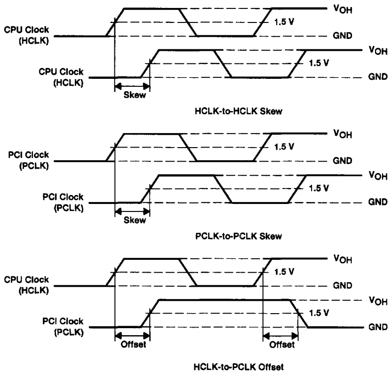
Figure 2. Waveforms for Calculation of t_{skew} and t_{offset}
