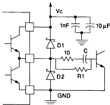
Power Bipolar Drive Circuit
