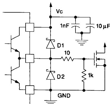
Power MOSFET Drive Circuit
