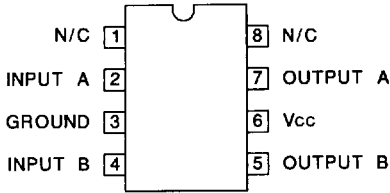
8 PIN DIL (TOP VIEW) N or J Package
