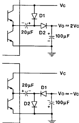
Charge Pump Circuits
