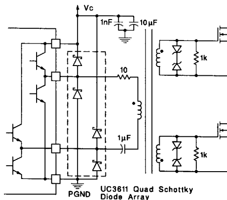
Transformer Coupled Push-Pull MOSFET Drive Circuit
