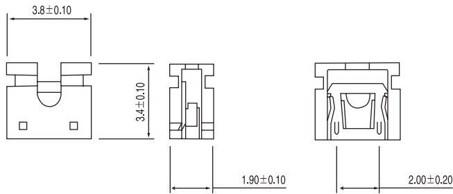
MJ-01 (2.0mm open. H: 3.4mm)
