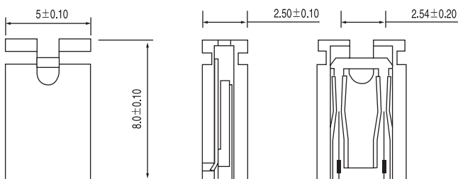
MJ-05 (2.54mm open. H: 8.0mm)
