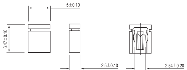
MJ-06 (2.54mm open)
