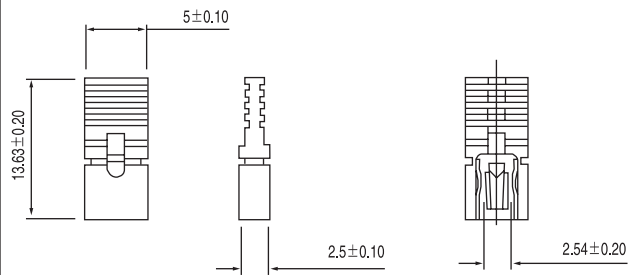
MJ-06 (2.54mm open)
