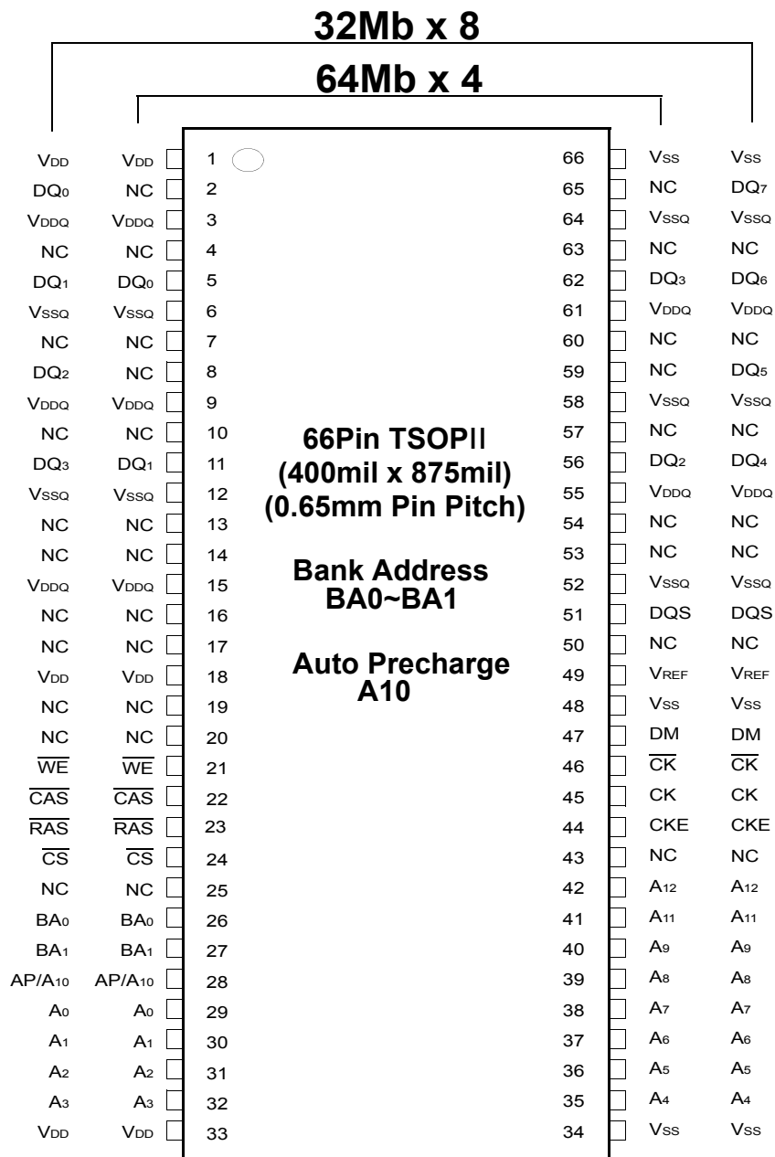
256Mb TSOP II Package Pinout
