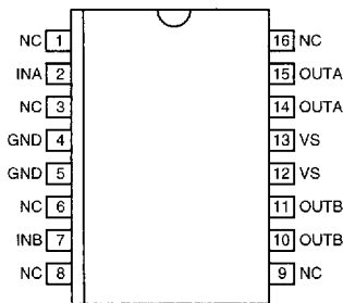
16-lead Wide SOIC (WM)
