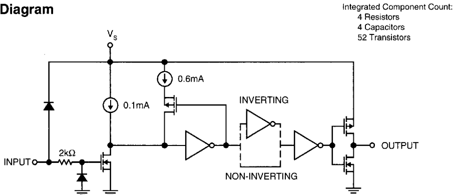
Functional Diagram for One Driver (Two Drivers per Package—Ground Unused Drivers)
