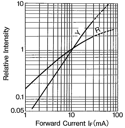
Fig.3 : Relative Intensity vs. Forward Current
