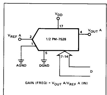
VOLTAGE SWITCHING MODE TEST CIRCUIT
