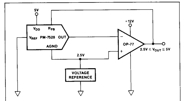
FIGURE 8: PM-7528 in Single Supply, Current-Steering Mode
