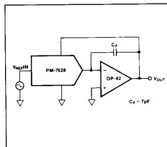
TEST CIRCUIT FOR GAIN vs FREQUENCY
