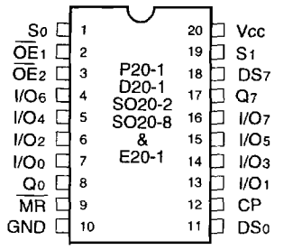
DIP/SOIC/QSOP/CERPACK TOP VIEW
