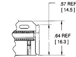
ASSEMBLED HEIGHT WITH STANDARD PLASTIC STRAIN RELIEF
