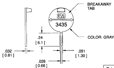
3435-0 KEYING PLUG (OPTIONAL: ORDER SEPARATELY)
