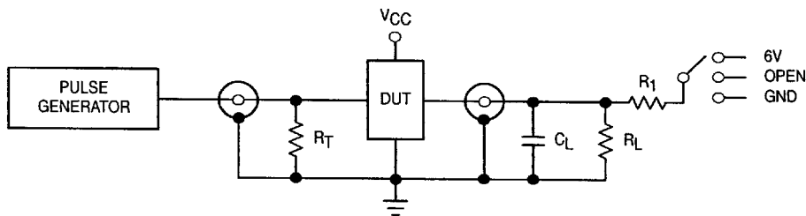
Figure 1. AC Waveforms
