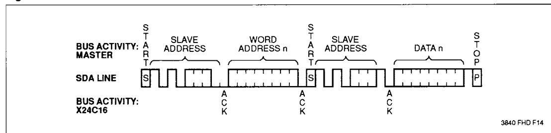
Figure 8. Random Read
