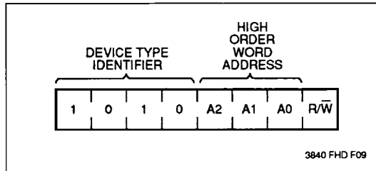
Figure 4. Slave Address
