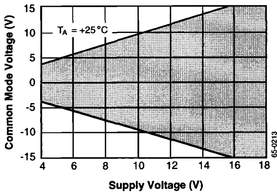
Common Mode Range vs. Supply Voltage
