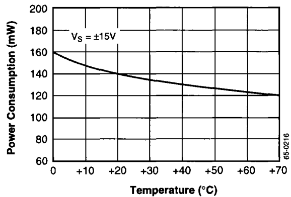
Power Consumption vs. Ambient Temperature
