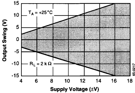
Typical Output Voltage vs. Supply Voltage
