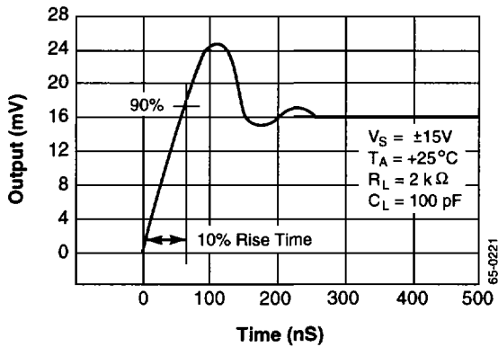
Transient Response
