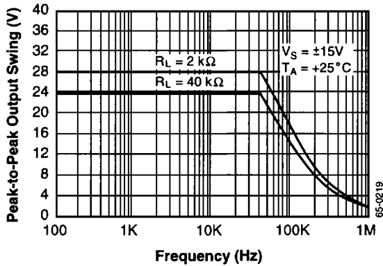
Output Voltage vs. Frequency
