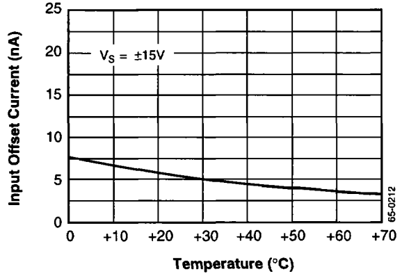
Input Offset Current vs. Ambient Temperature
