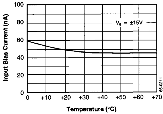
Input Bias Current vs. Ambient Temperature
