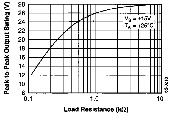
Output Voltage Swing vs. Load Resistance
