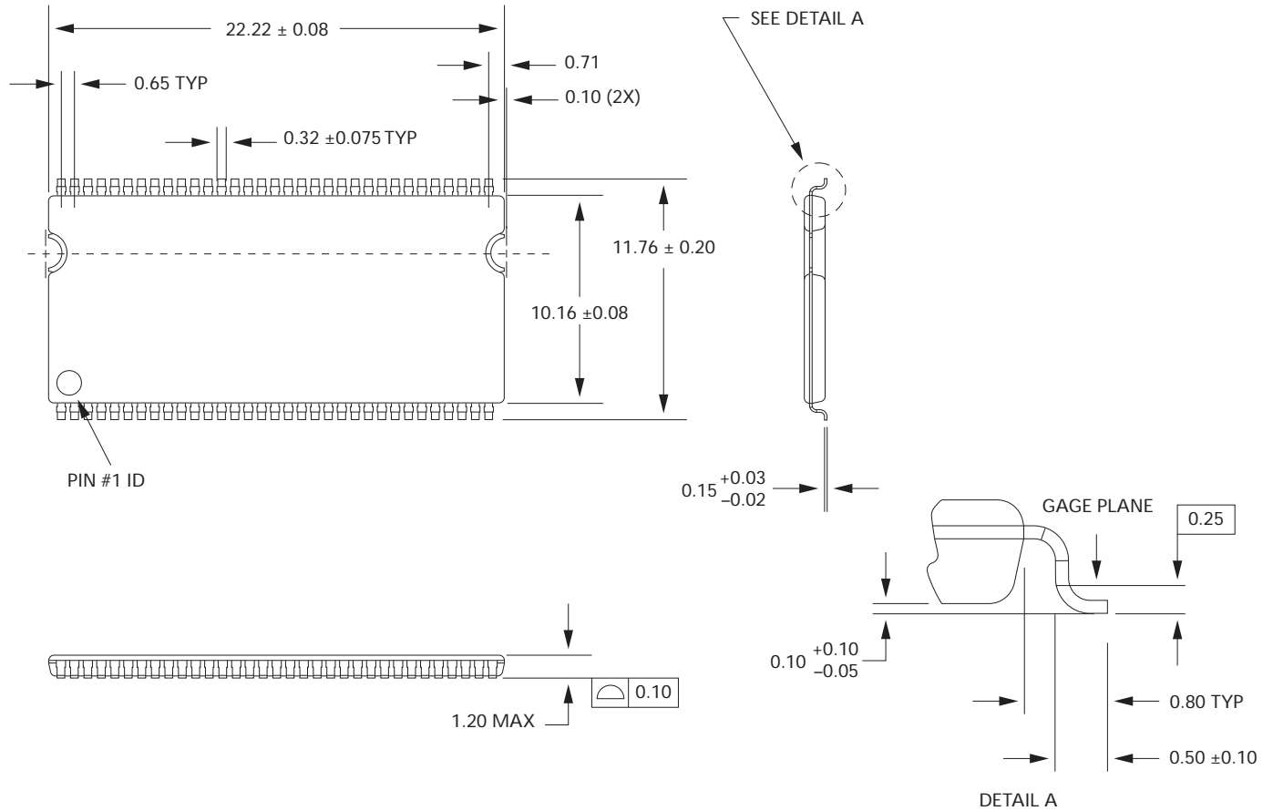
Figure 6: 66-Pin Plastic TSOP (400 mil)
