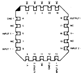
Leadless Chip-Pak L-20-1
