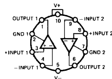
Metal Can H-10-1
