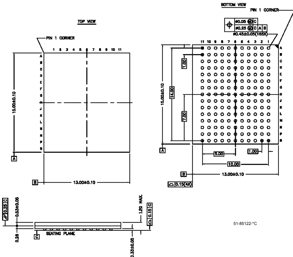
165-ball FBGA (13 x 15 x 1.2 mm) BB165A
