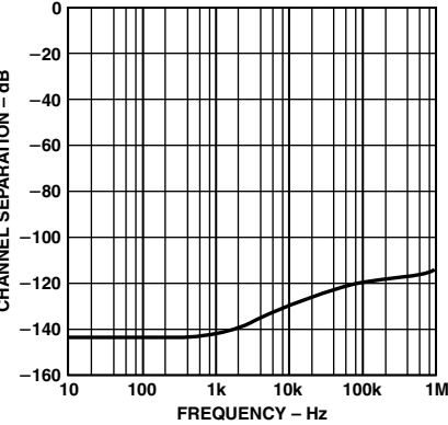
TPC 44. Channel Separation vs. Frequency
