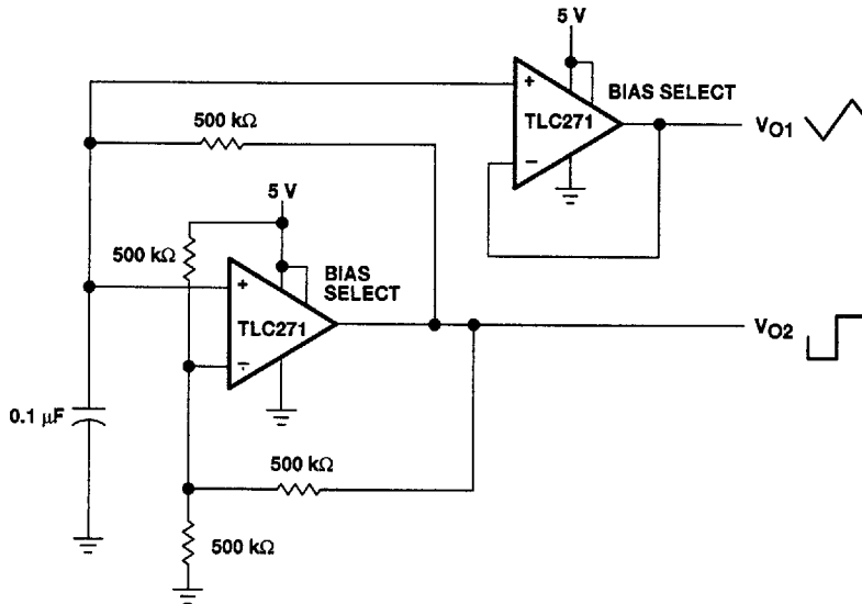
Figure 126. Multivibrator
