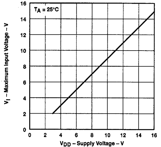
MAXIMUM INPUT VOLTAGE vs SUPPLY VOLTAGE
