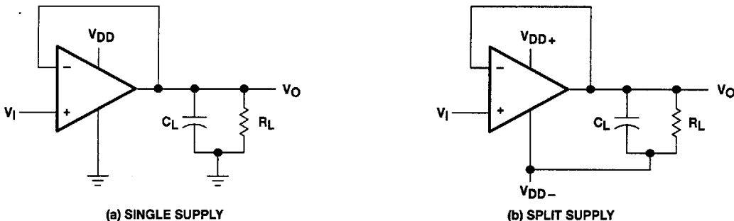
Figure 98. Unity-Gain Amplifier
