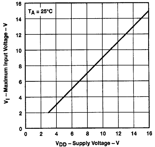
MAXIMUM INPUT VOLTAGE vs SUPPLY VOLTAGE
