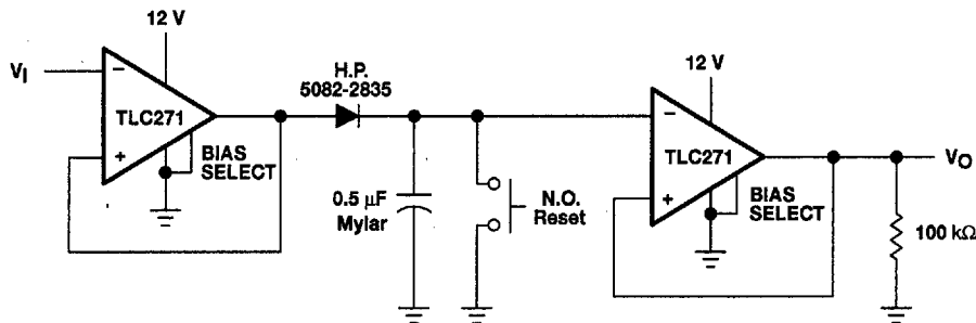
Figure 119. Positive-Peak Detector
