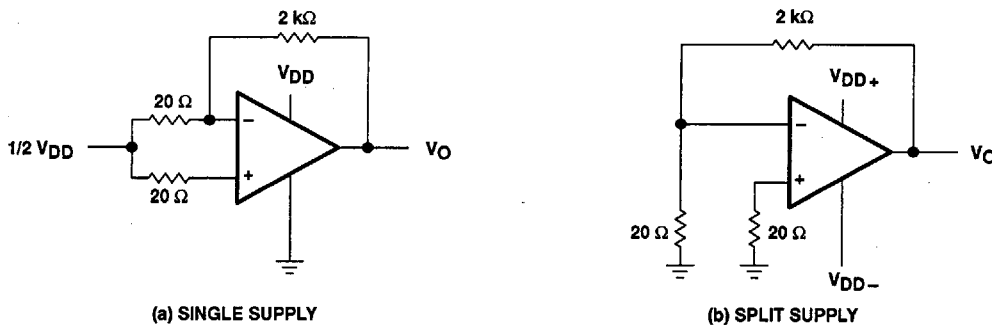
Figure 99. Noise-Test Circuit
