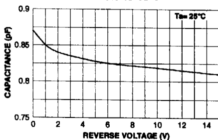
CAPACITANCE vs REVERSE VOLTAGE VR = 0.0 to 15 V
