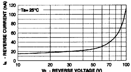
REVERSE CURRENT vs REVERSE VOLTAGE IR - 10 to 100 V
