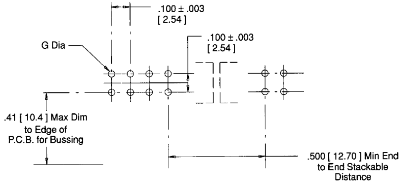
RECOMMENDED Mounting Hole Pattern
