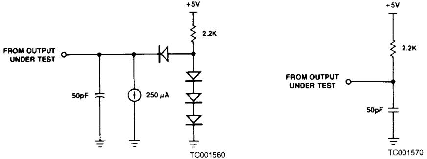
B. Open-Drain Test Load
