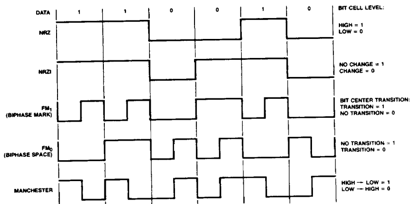
Figure 4. Data Encoding Methods
