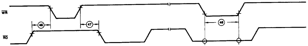
Figure 22. Z8531 Reset Timing
