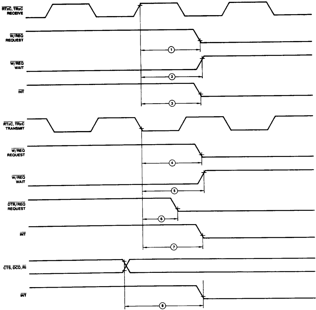
Figure 14. System Timing
