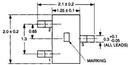
PACKAGE OUTLINE 30
