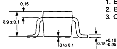
PACKAGE OUTLINE 33
