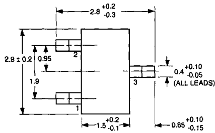
PACKAGE OUTLINE 33
