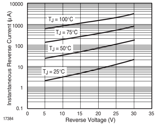
Fig. 6 Typical Reverse Current Characteristics - SL03
