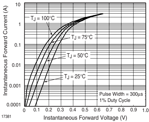
Fig. 3 Typical Instantaneous Forward Characteristics - SL02
