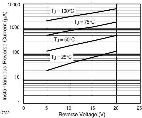
Fig. 4 Typical Reverse Current Characteristics - SL02
