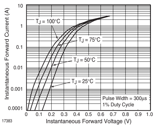
Fig. 5 Typical Instantaneous Forward Characteristics - SL03
