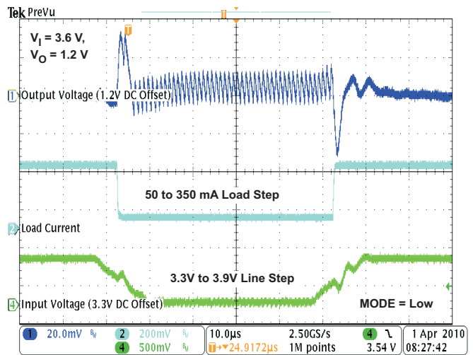
COMBINED LINE/LOAD TRANSIENT RESPONSE
