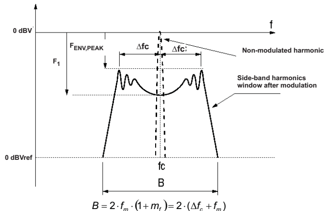
Figure 40. Spectrum of a Frequency Modulated Sin. Wave with Sinusoidal Variation in Time
