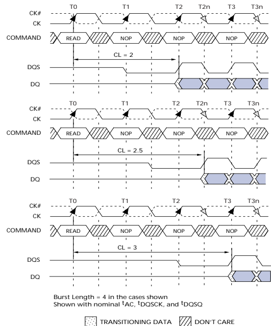
Figure 8: CAS Latency
