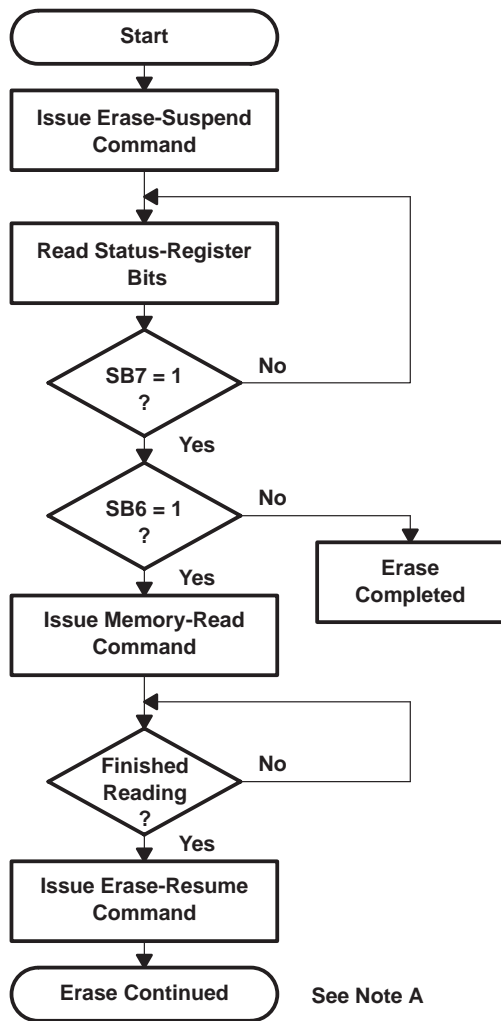
Figure 6. Erase-Suspend/Eraser-Resume Flow Chart
