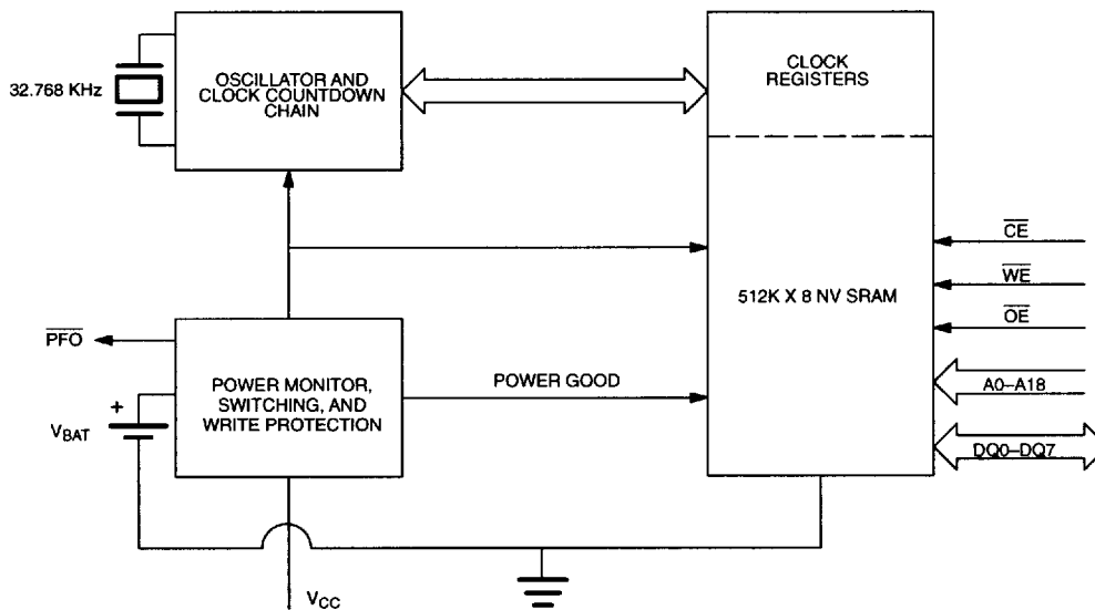
BLOCK DIAGRAM DS1647 Figure 1
