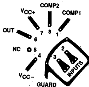
Figure 14. Input Guarding
