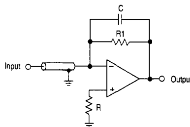
Figure 17. Cable Bootstrapping and Input Shields
