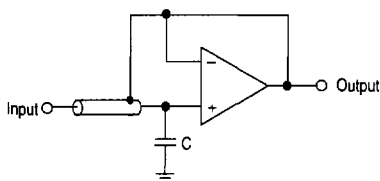
Figure 17. Cable Bootstrapping and Input Shields
