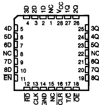
SN54ALS996 ... FK PACKAGE (TOP VIEW)
