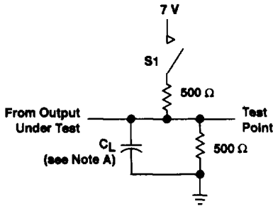
LOAD CIRCUIT FOR Q OUTPUTS
