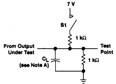
LOAD CIRCUIT FOR D OUTPUTS
