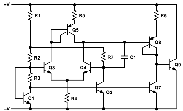
Figure 4. Schematic Diagram
