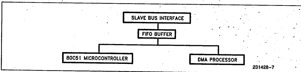
Figure 3. UPI-452 Conceptual Block Diagram
