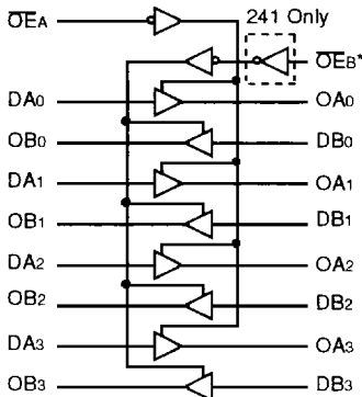
IDT54/74FCT241/244
