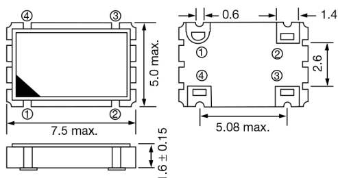
Figure 1) ECS-3951M/3953M Top, Side and Bottom views
