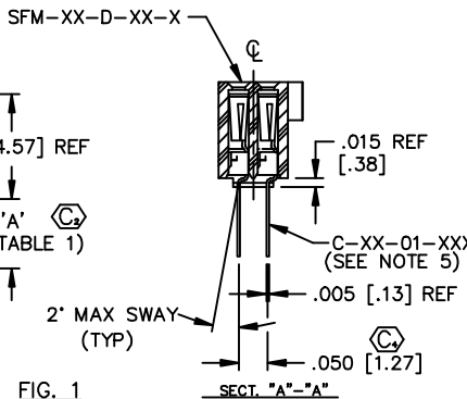
FIG. 1 THROUGH HOLE/STRAIGHT MODIFIED
