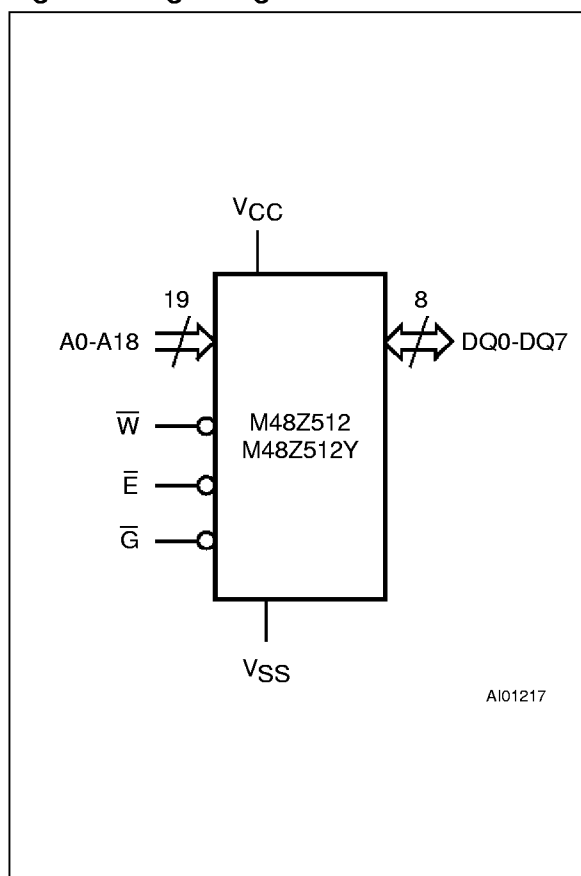
Figure 1. Logic Diagram
