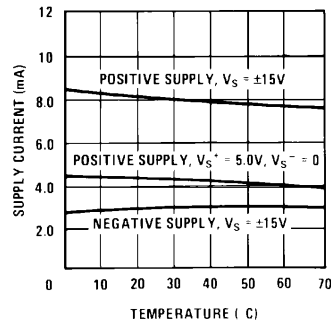
Supply Currents
