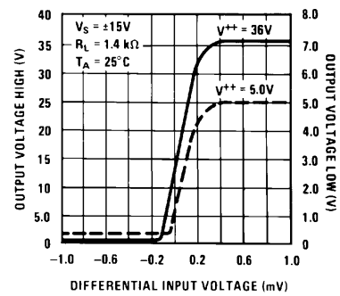
Transfer Function
