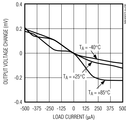
MAX6023EBK50 LOAD REGULATION
