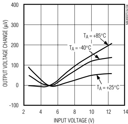
MAX6023EBK12 LINE REGULATION
