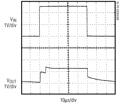
MAX6023EBK12 TURN-ON TRANSIENT
