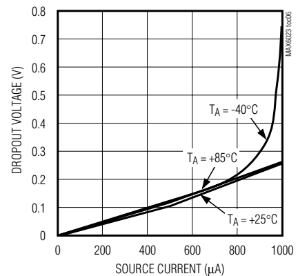
MAX6023EBK41/45/50 DROPOUT VOLTAGE vs. SOURCE CURRENT
