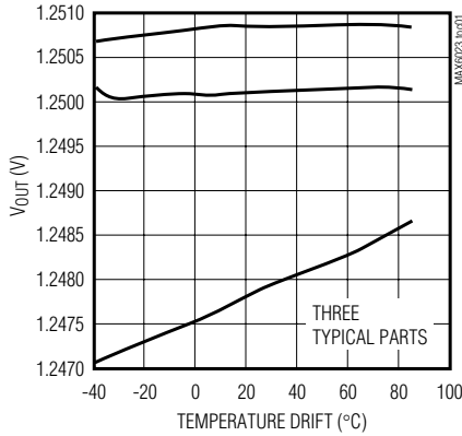
MAX6023EBK12 OUTPUT VOLTAGE TEMPERATURE DRIFT
