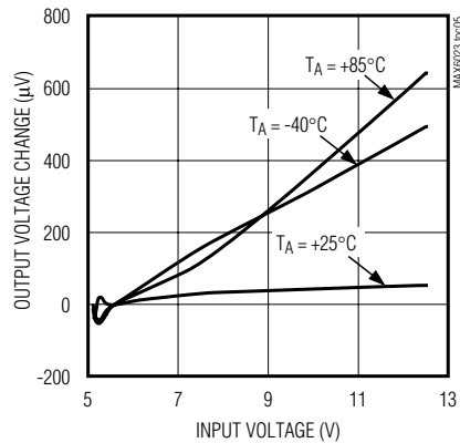
MAX6023EBK50 LINE REGULATION
