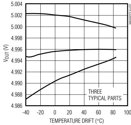
MAX6023EBK50 OUTPUT VOLTAGE TEMPERATURE DRIFT
