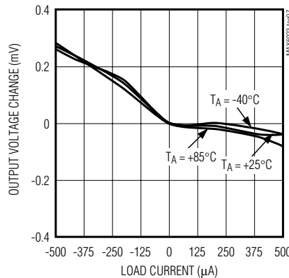
MAX6023EBK12 LOAD REGULATION
