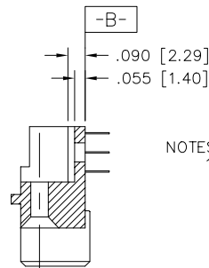
SECTION W-W
