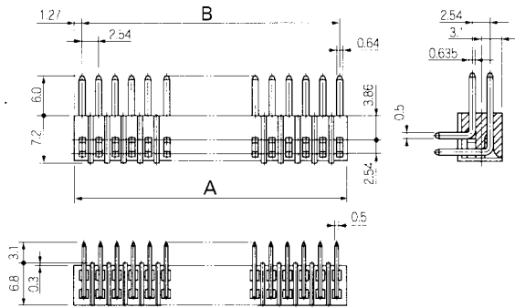
Terminal Type 2 - Right Angle Solder Dip
