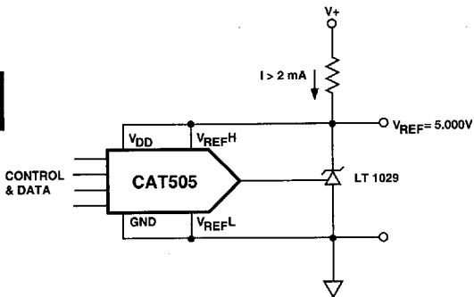
Digitally Trimmed Voltage Reference
